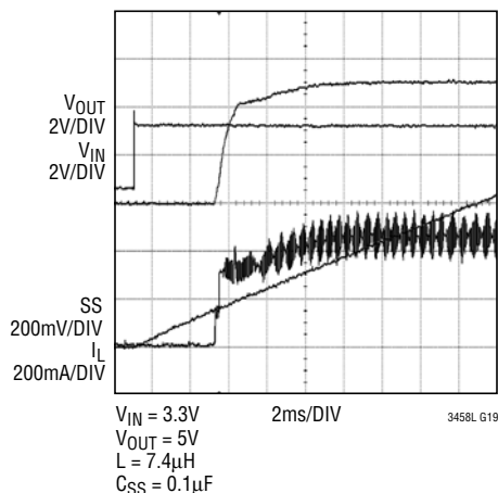
Soft-Start into 20\Omega Load
